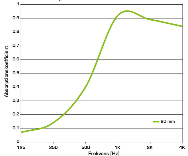
Absorptionskoefficient iht. DIN 52 215
